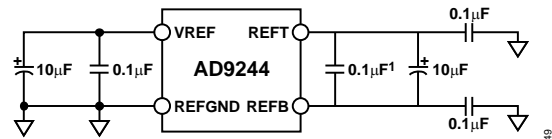
*LOCATE AS CLOSE AS POSSIBLE TO REFT/REFB PINS.
